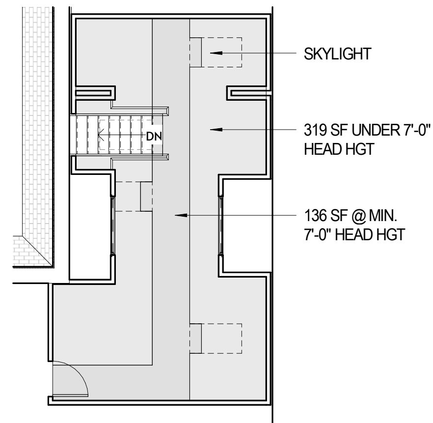
② Attic/loft Floor - Suite 2 1/8" = 1'-0"
