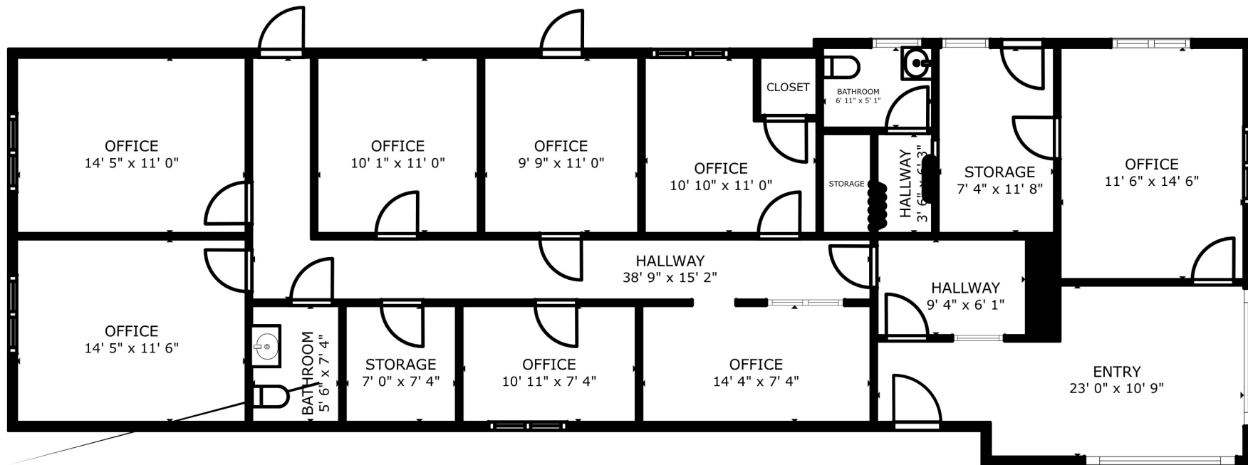
FLOOR PLAN
