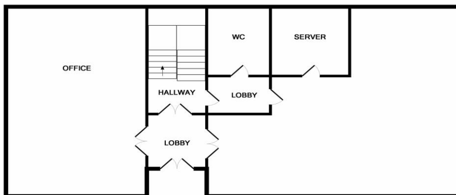
GROUND FLOOR
