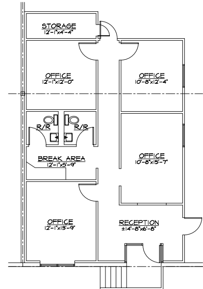
ENLARGED OFFICE PLAN
