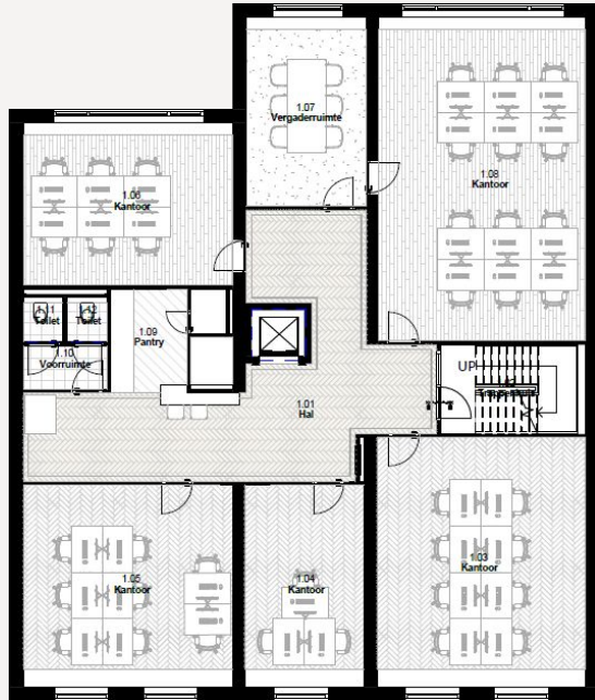
Floor 1
