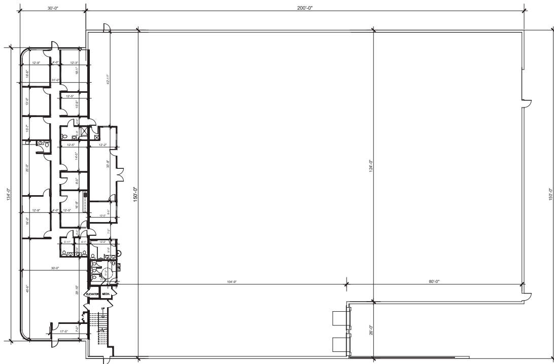
FIRST LEVEL FLOOR PLAN
