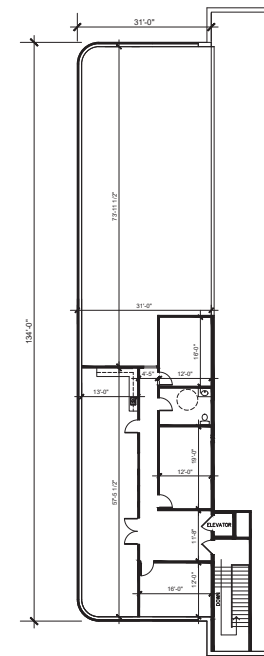
SECOND LEVEL FLOOR PLAN
