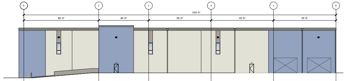
WEST ELEVATION 1/16" = 1'-0"
