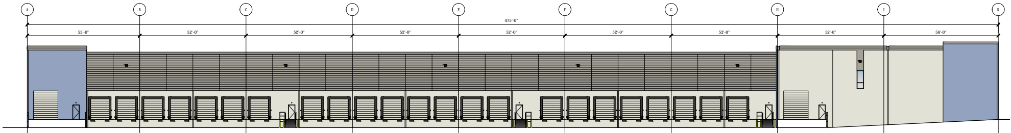
NORTH ELEVATION 1/16" = 1'-0"
