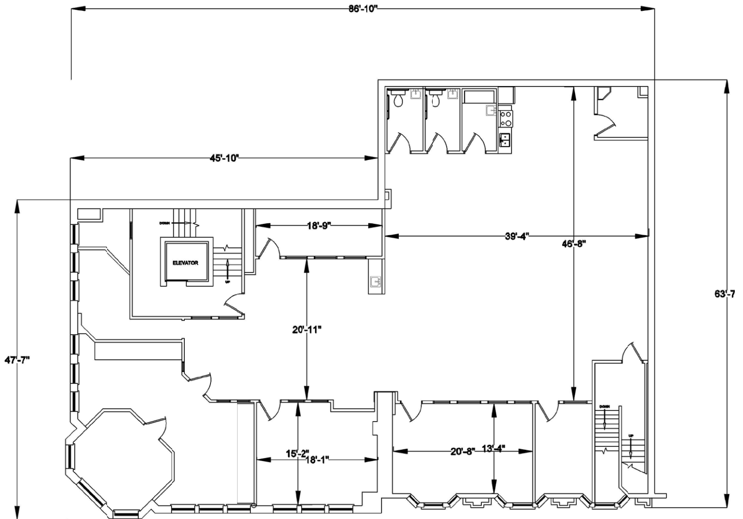
THIRD FLOOR
