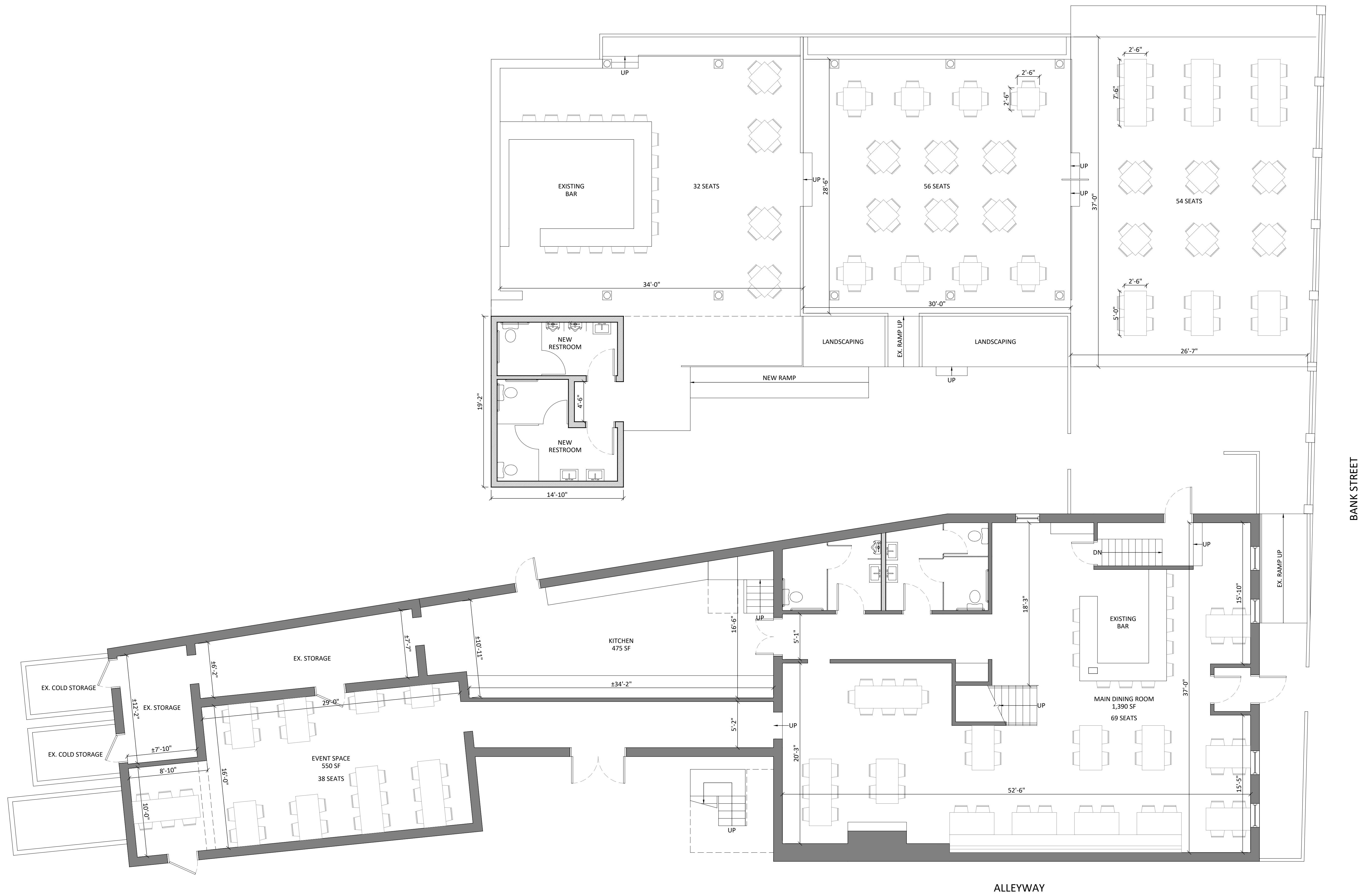
1 PROPOSED 1ST FLOOR PLAN 3/16" = 1'-0"
