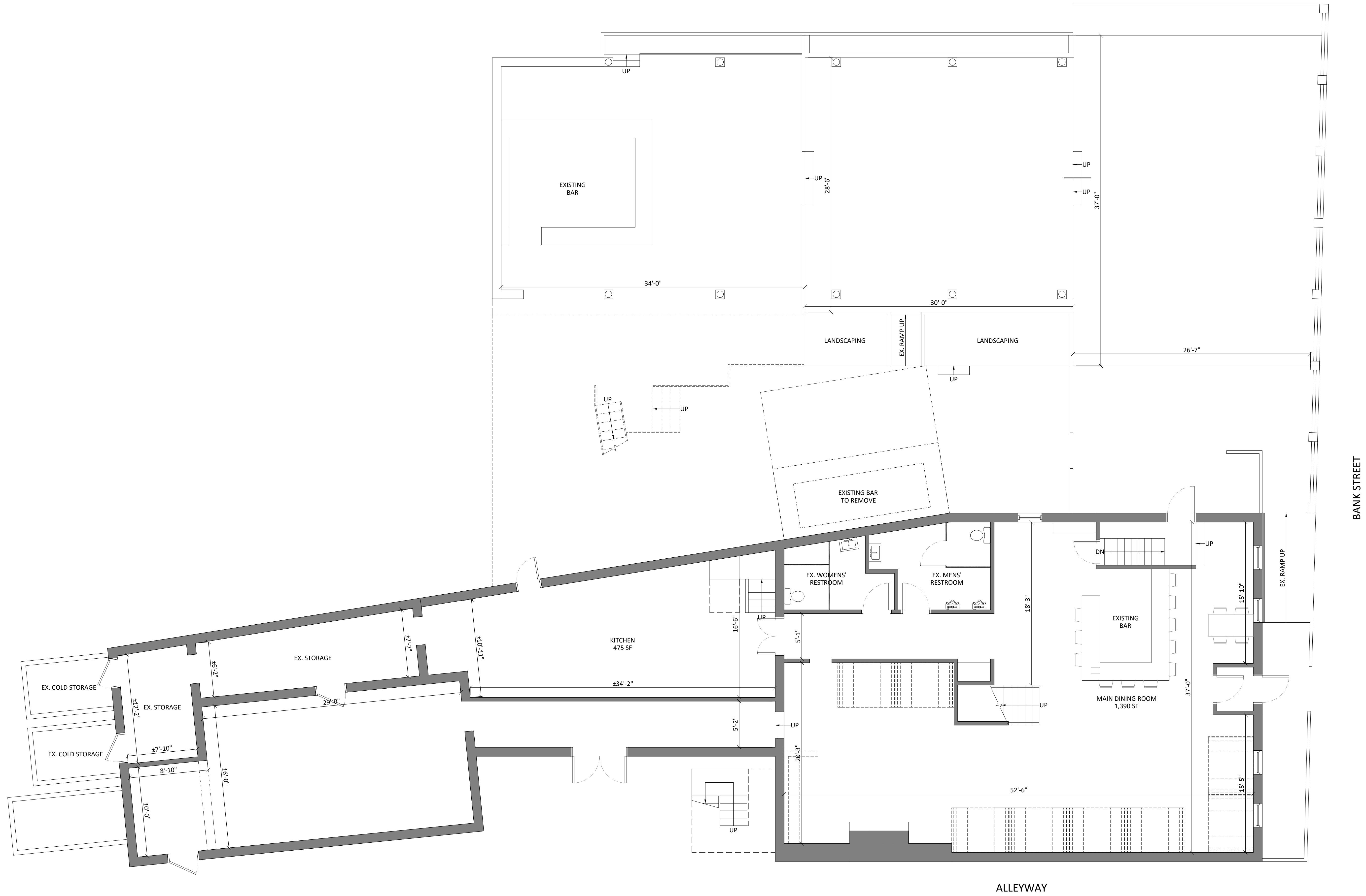
1 EXISTING 1ST FLOOR PLAN 3/16" = 1'-0"
