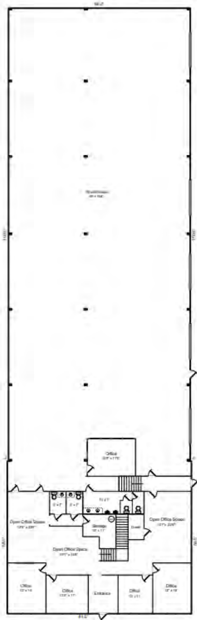
Warehouse First Floor 9672.3sf
