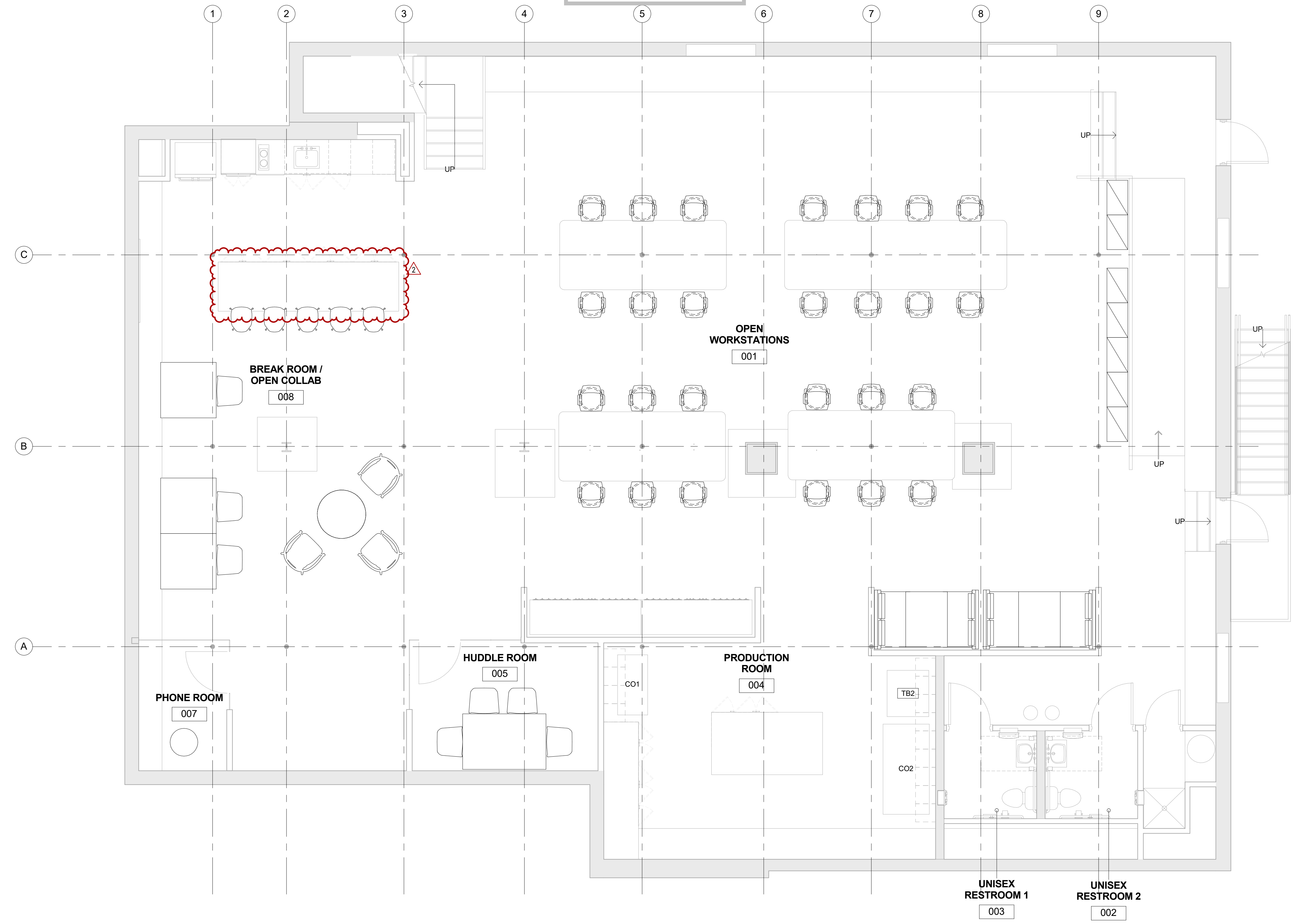
1 FURNITURE PLAN LEVEL 00 A901 1/4" = 1'-0"
