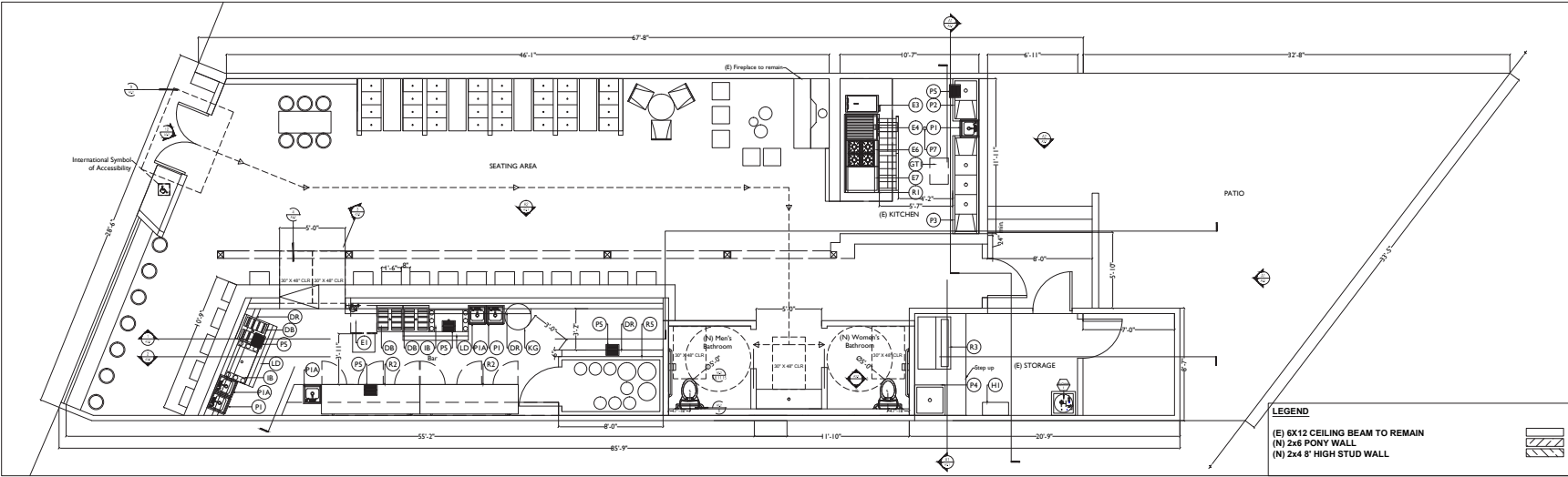
New Floor Plan Scale: 1/4" = 1'
