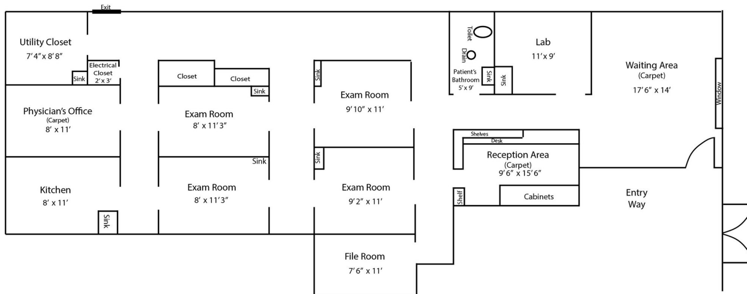
1 FIRST FLOOR PLAN 2,300 SF Medical Office
