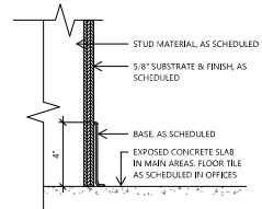
7 TYP. BASE DETAIL
