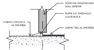
3 CARPET AND CONCRETE TRANSITION AT OFFICES
