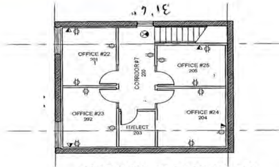
SECOND FLOOR PLAN SCALE: 3/32" = 1'-0"
