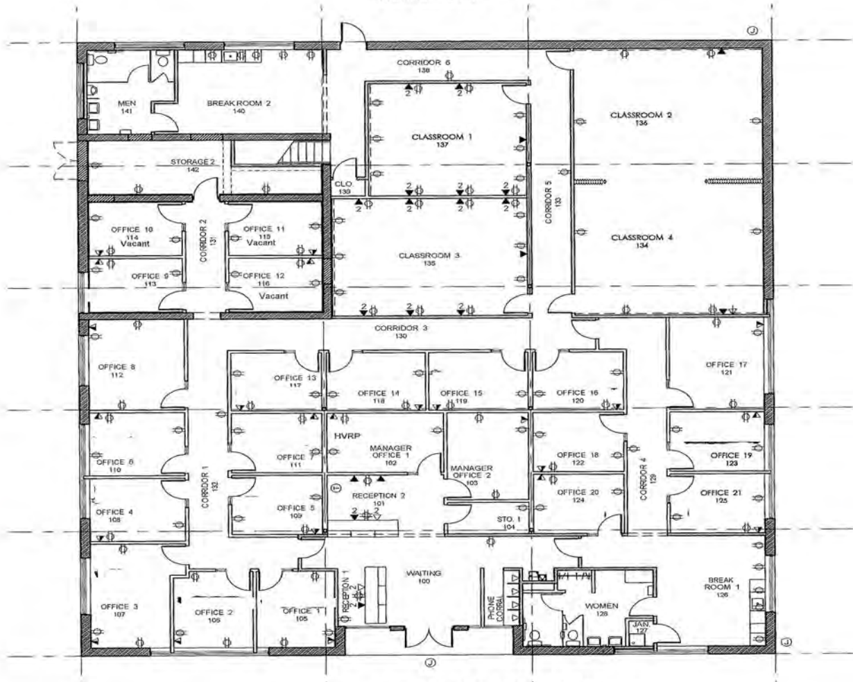
FIRST FLOOR PLAN SCALE: 3/32" = 1'-0"
