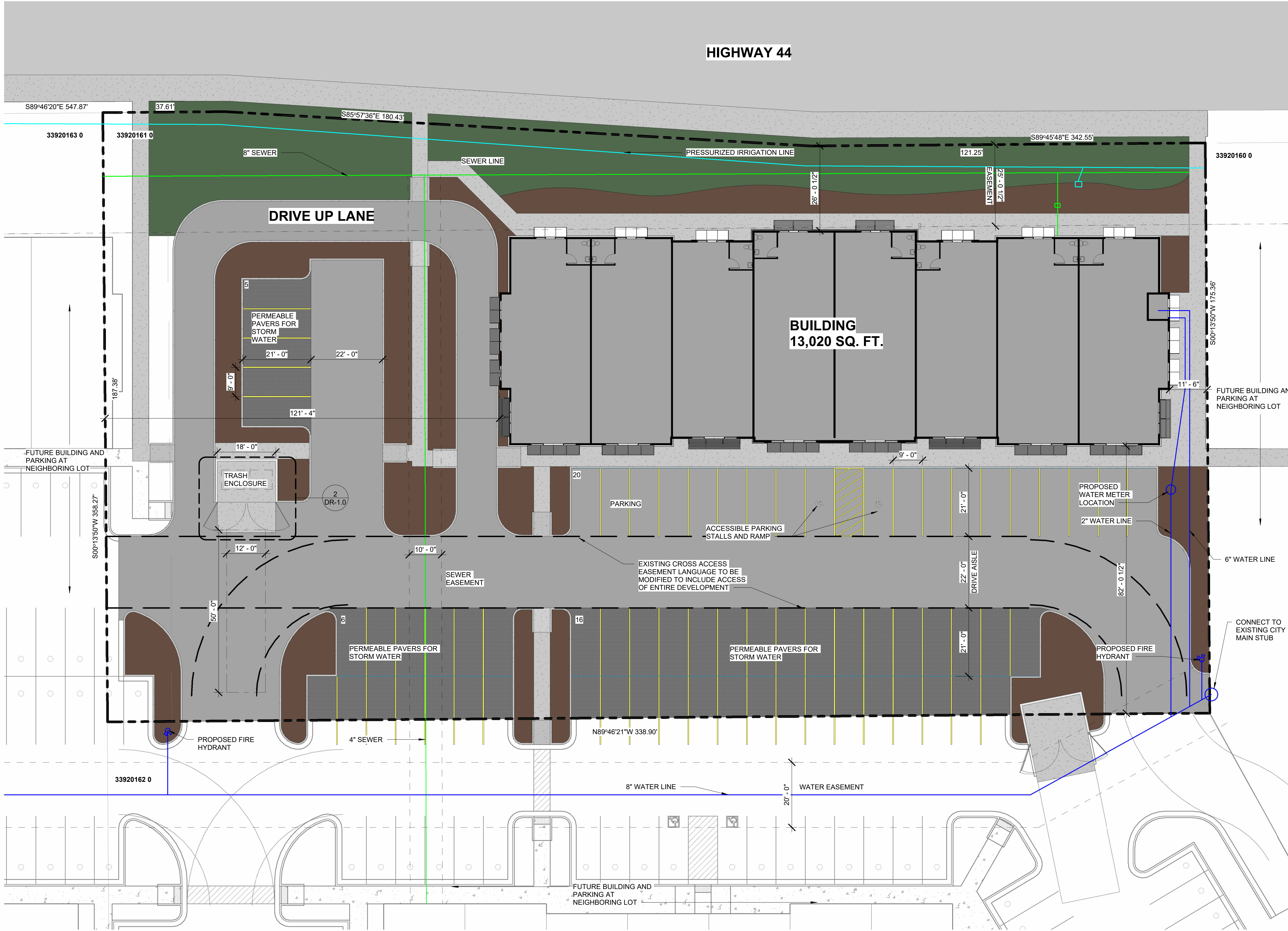
1 SITE PLAN 1/16" = 1'-0"
