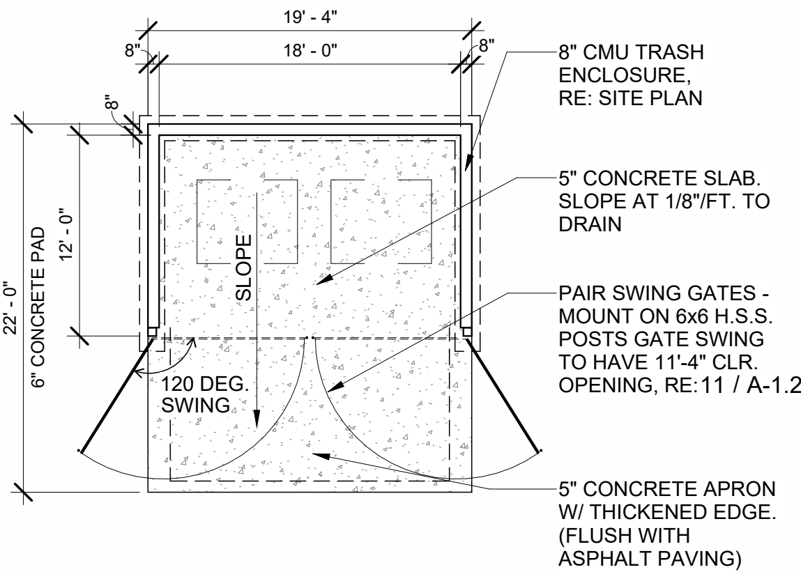
2 TRASH ENCLOSURE - PLAN 1/8" = 1'-0"
