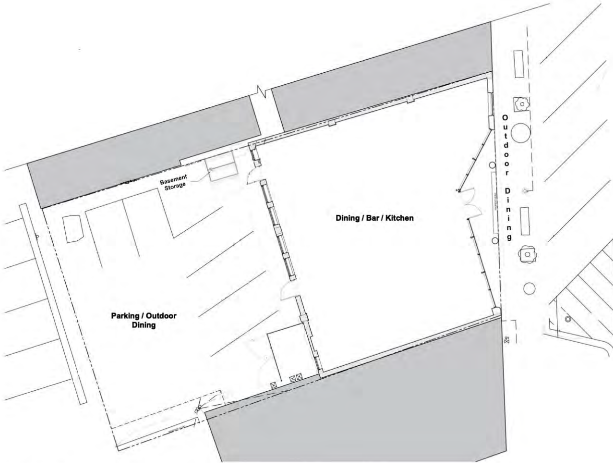
1 SITE PLAN 1/8" = 1'-0"
