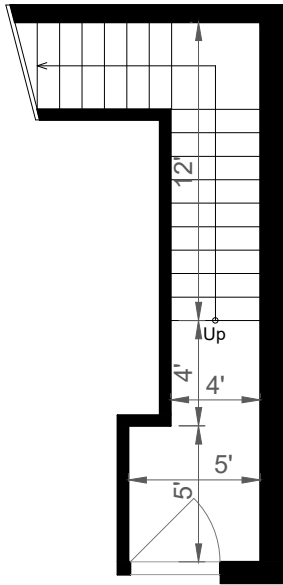
FIRST FLOOR 150 SQ FT
