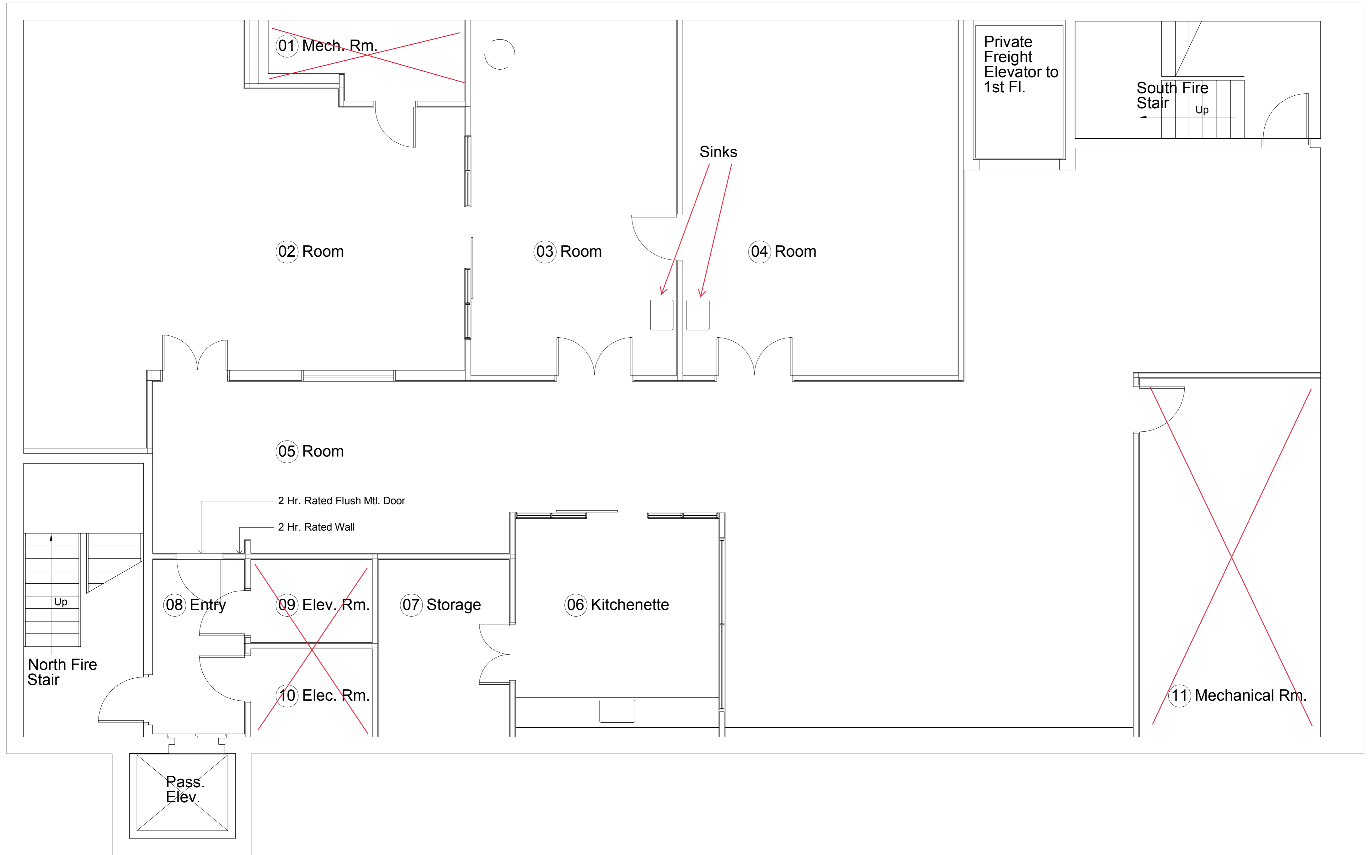
1 Basement Plan Scale 1/4"=1'-0"
