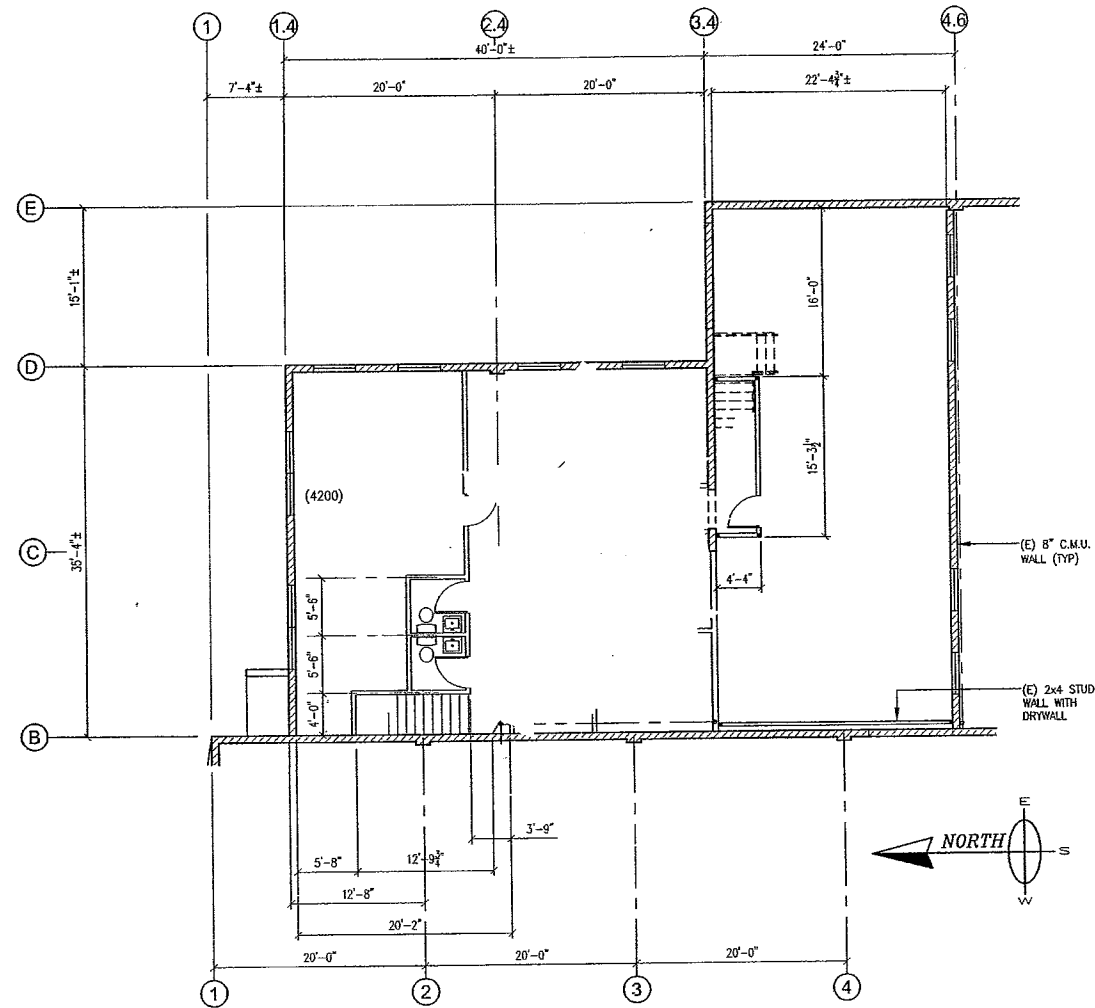
EXISTING SECOND FLOOR PLAN SCALE: 1/8" = 1'-0"
