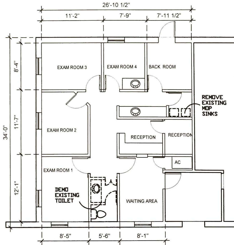
01 EXISTING SUITE A-FLOOR PLAN 1/8" : 1'-0" 890 SF
