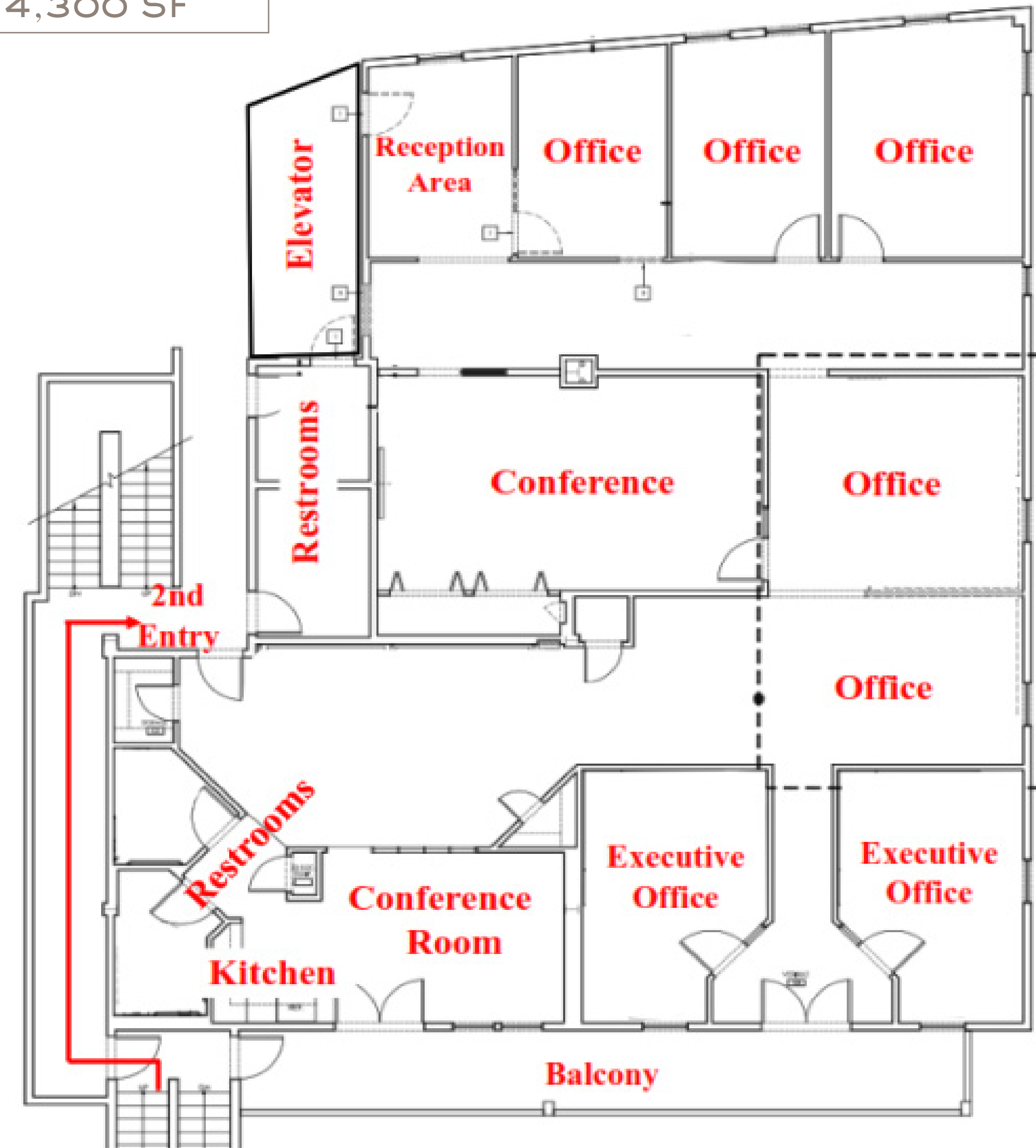
FLOOR PLAN
