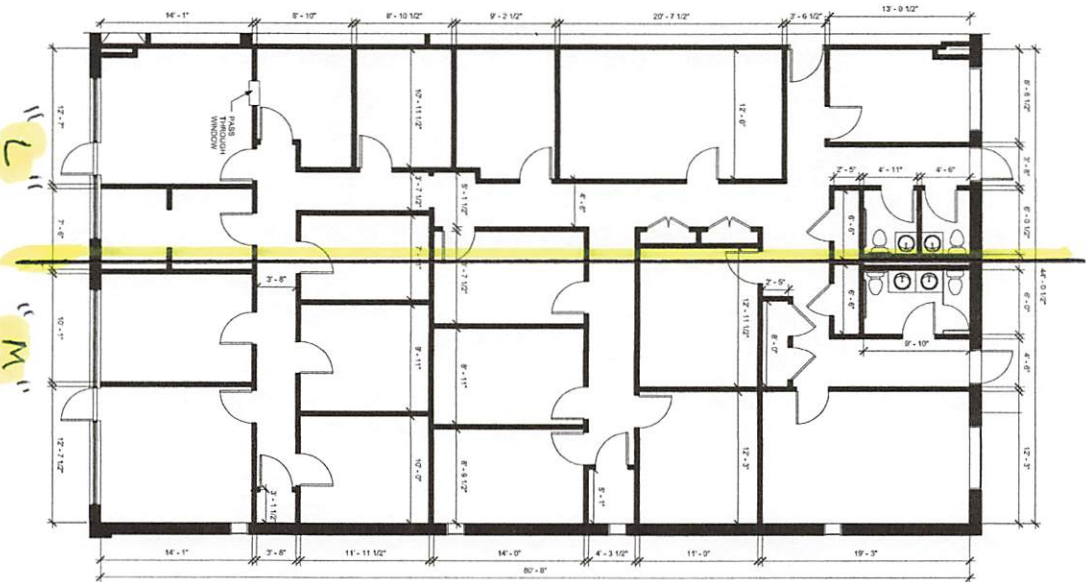
2 FLOOR PLAN - TENANT SPACE 3 SIB = 1/8"
