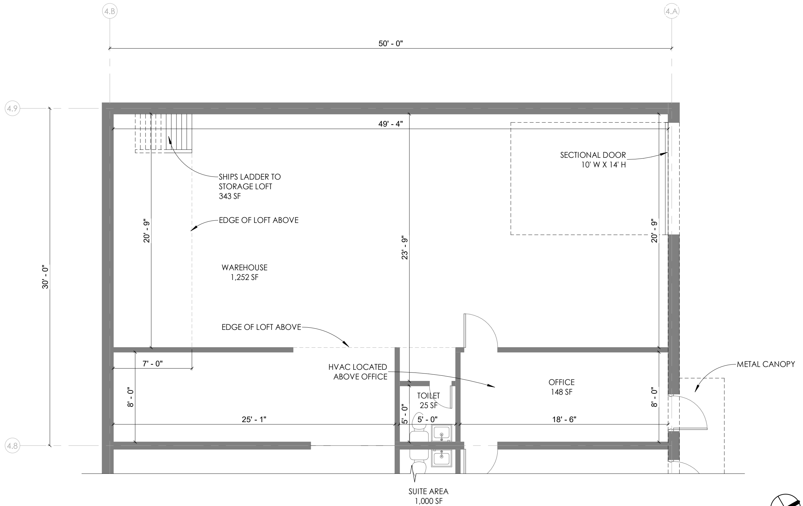
1 SUITE 108 - EXISTING FLOOR PLAN - 1,500 SF 3/16" = 1'-0"
