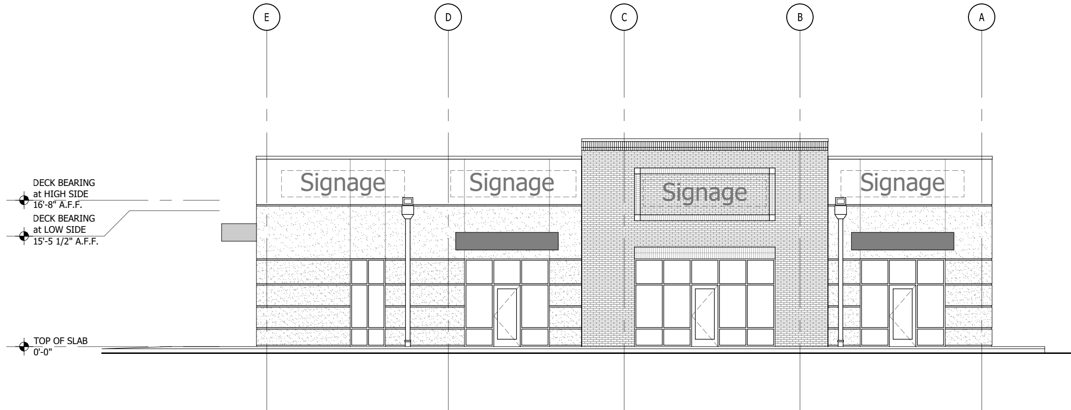
2 EAST ELEVATION
