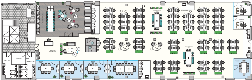
INDICATIVE SPACE PLAN
