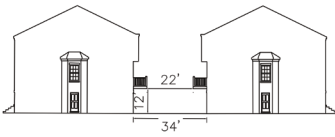
TYPICAL ALLEY CROSS SECTION
