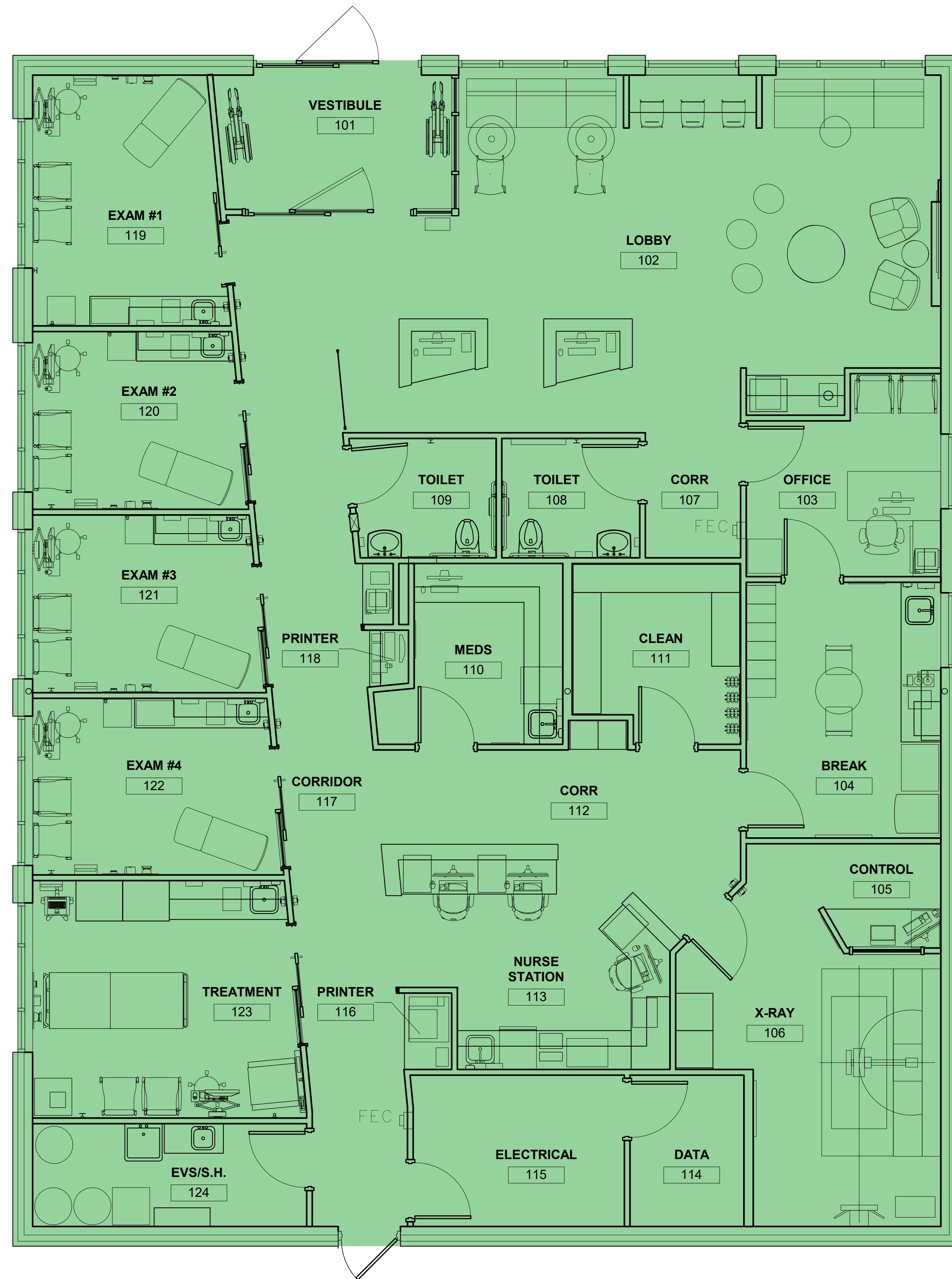
1 GROSS BUILDING AREA PLAN - FIRST FLOOR 1/4" = 1'-0"
