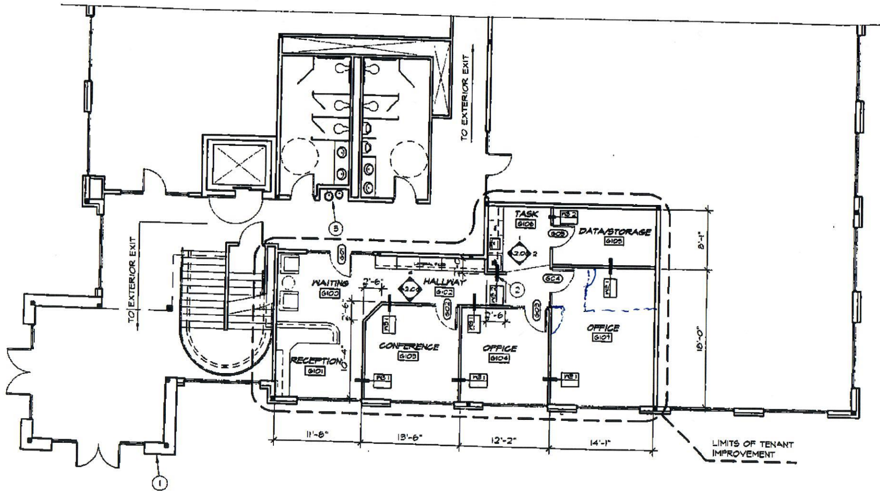
A Partial Ground Level Floor Plan Scale: 1/8" = 1'-0"
