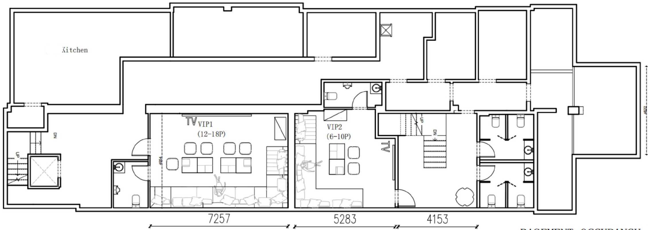
BASEMENT OCCUPANCY 1 (finish ceiling height 2641mm)
