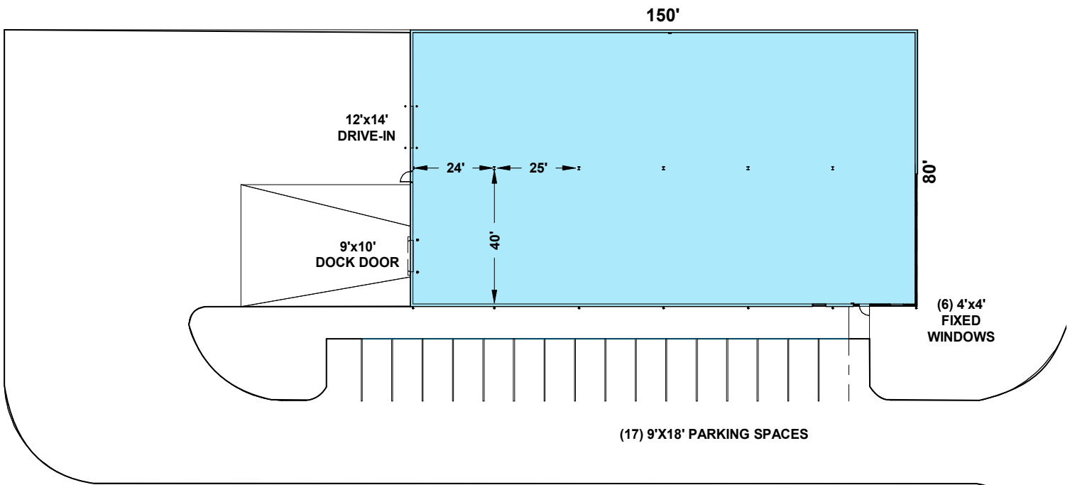
SITE PLAN
