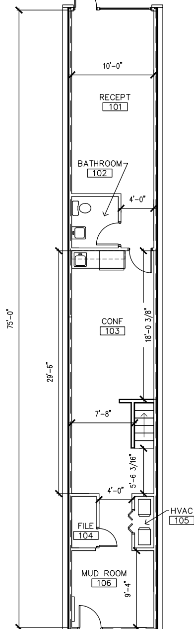
OFFICE FLOOR PLAN 750 SF
