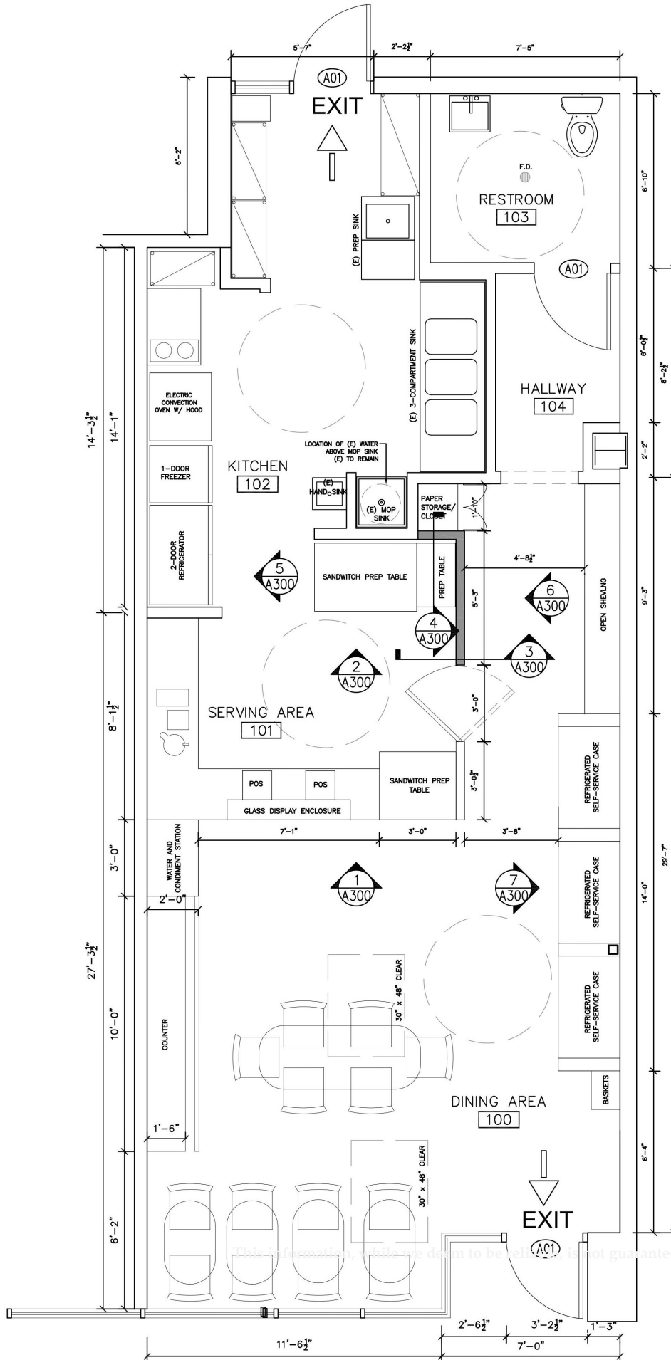
252 S Beverly Drive Floor Plan
