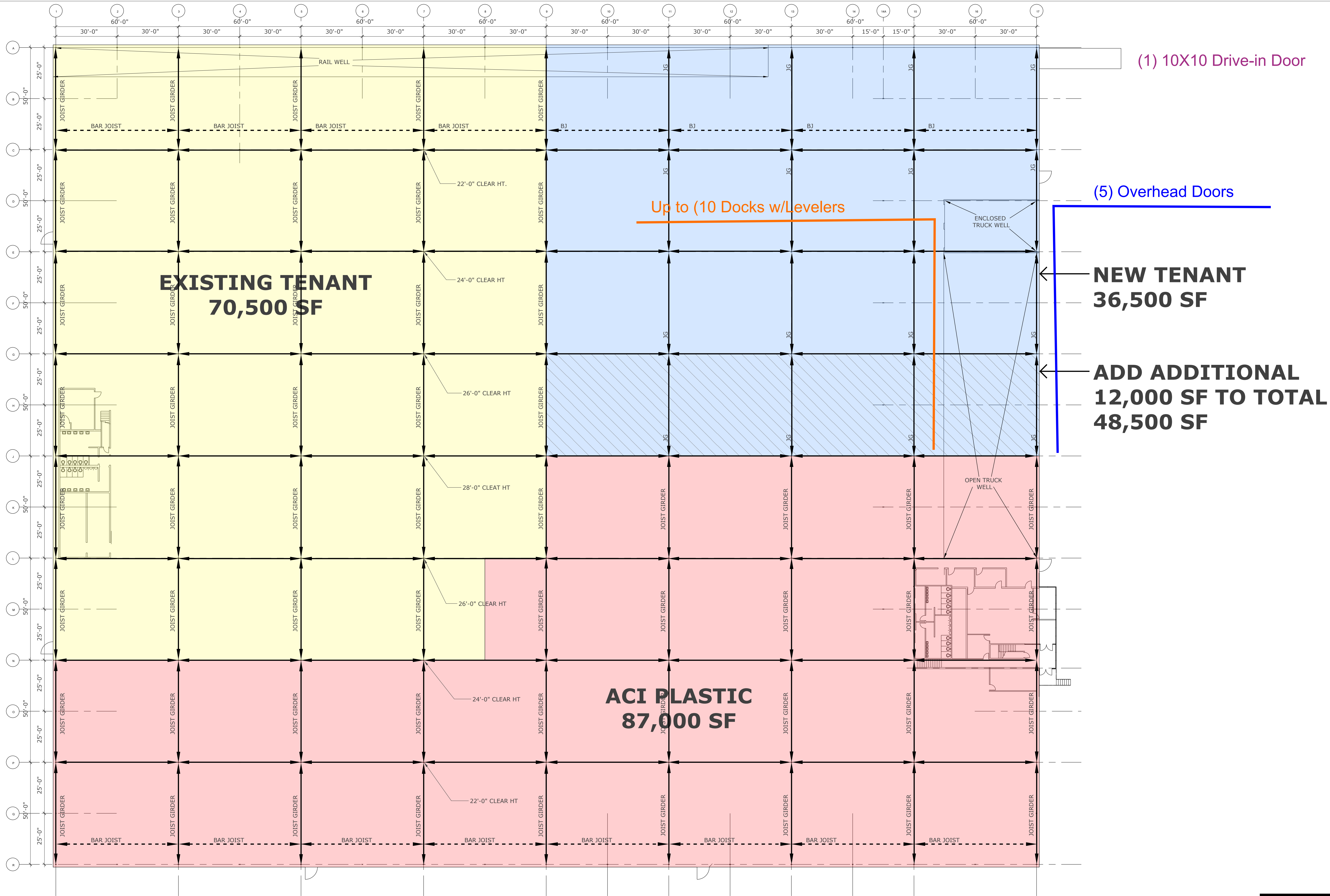
0 PLANT FLOOR PLAN Scale: 1" : 10'
