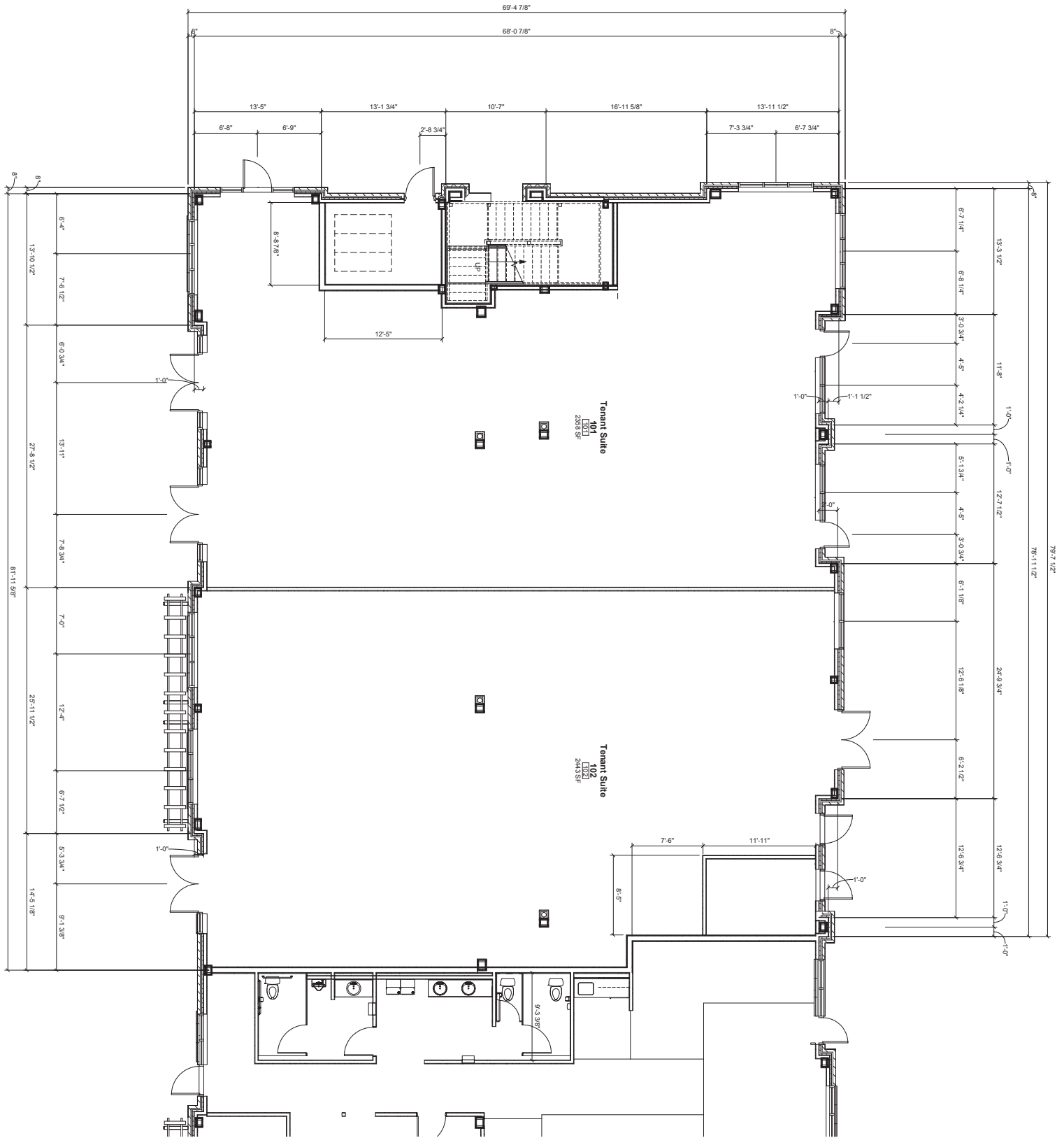
FLOOR PLAN - 2
