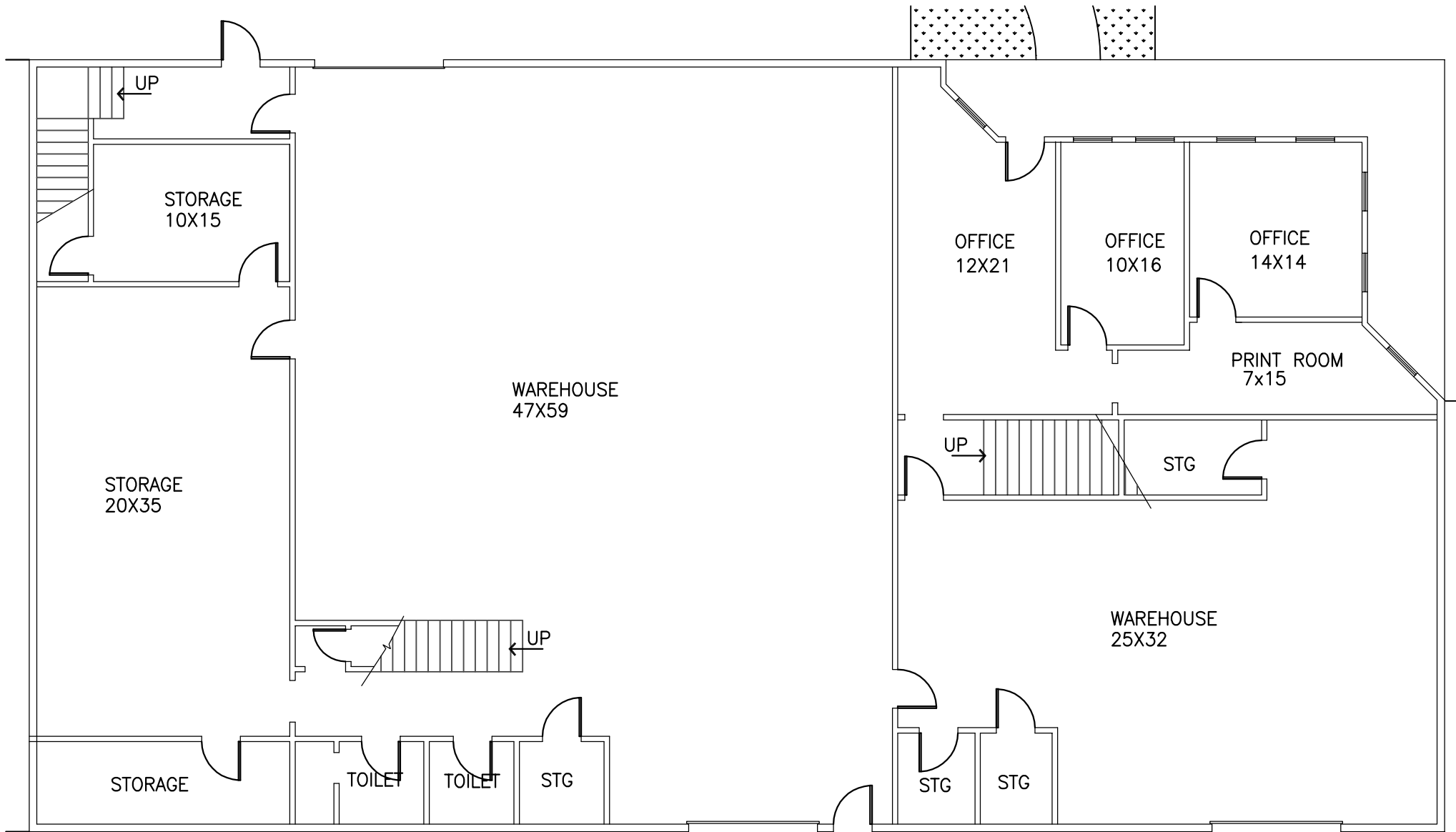
GROUND LEVEL FLOOR PLAN 3/32"=1'-0"
