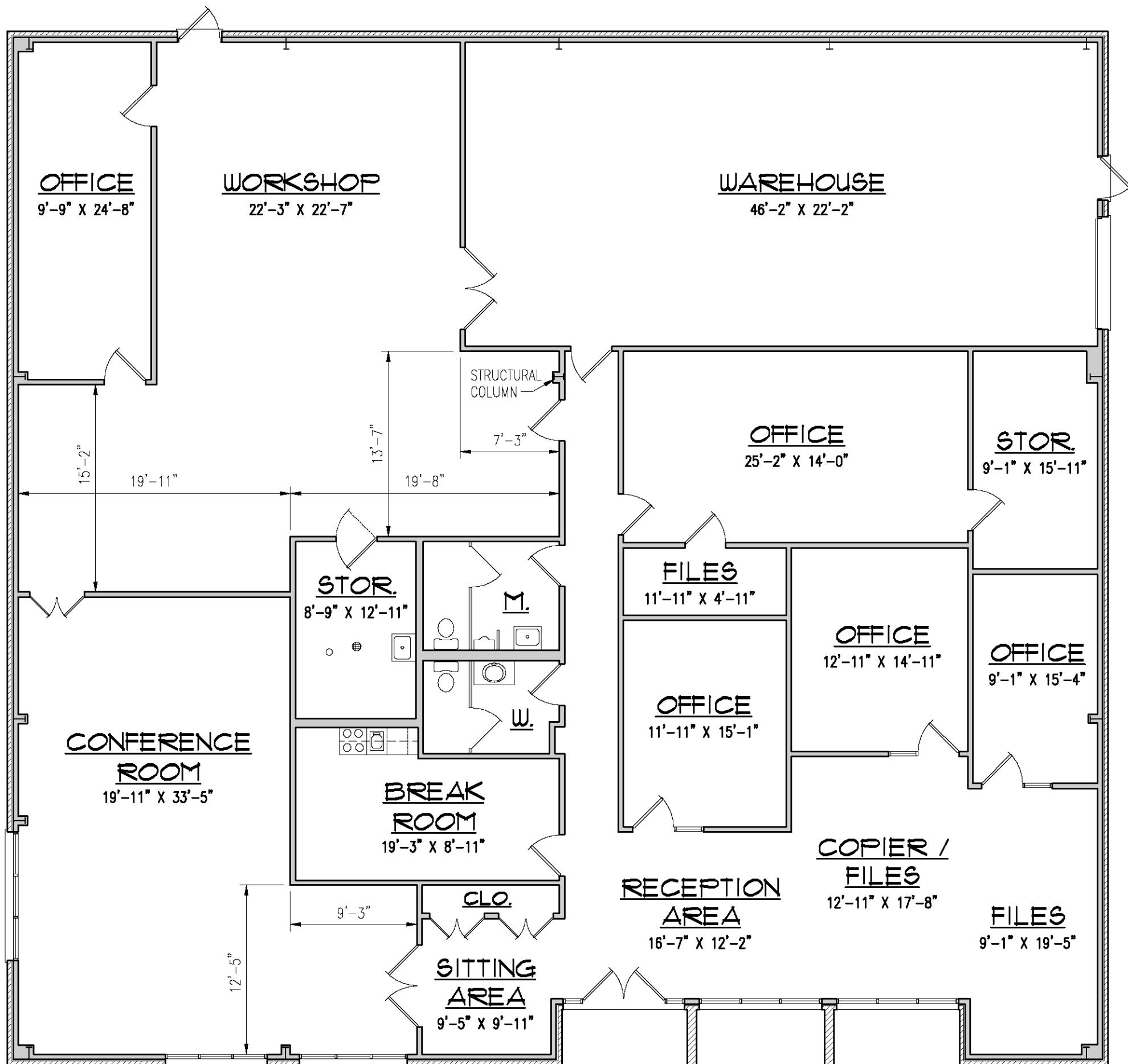
FLOOR PLAN
