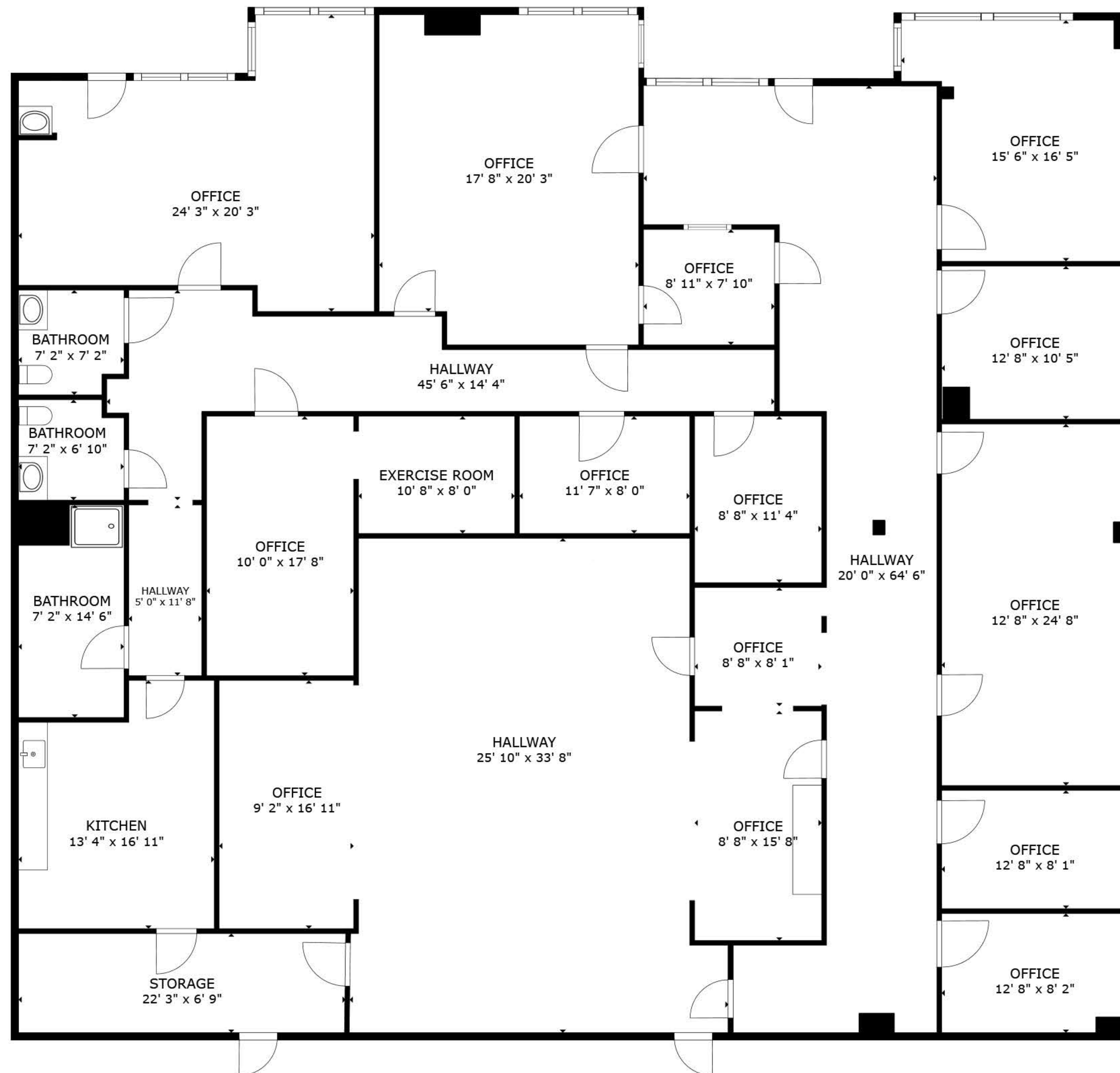
FLOOR PLAN
