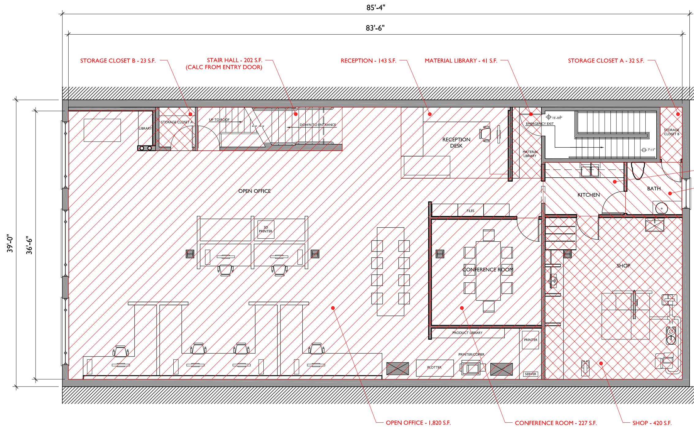
KA OFFICE PLAN AT SECOND LEVEL 1/4" = 1'-0"
