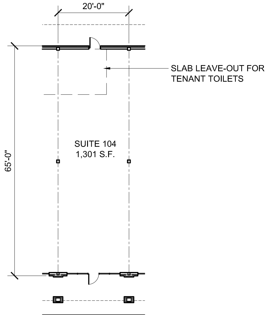
LEASING PLAN - SUITE 104
