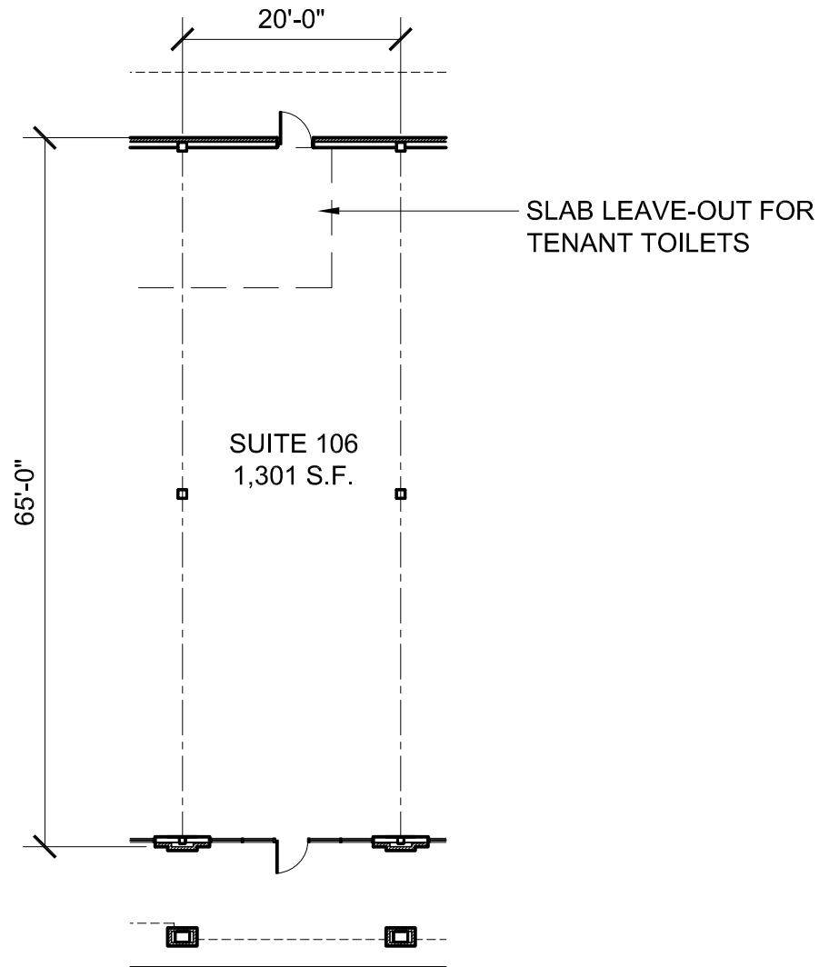
LEASING PLAN - SUITE 106
