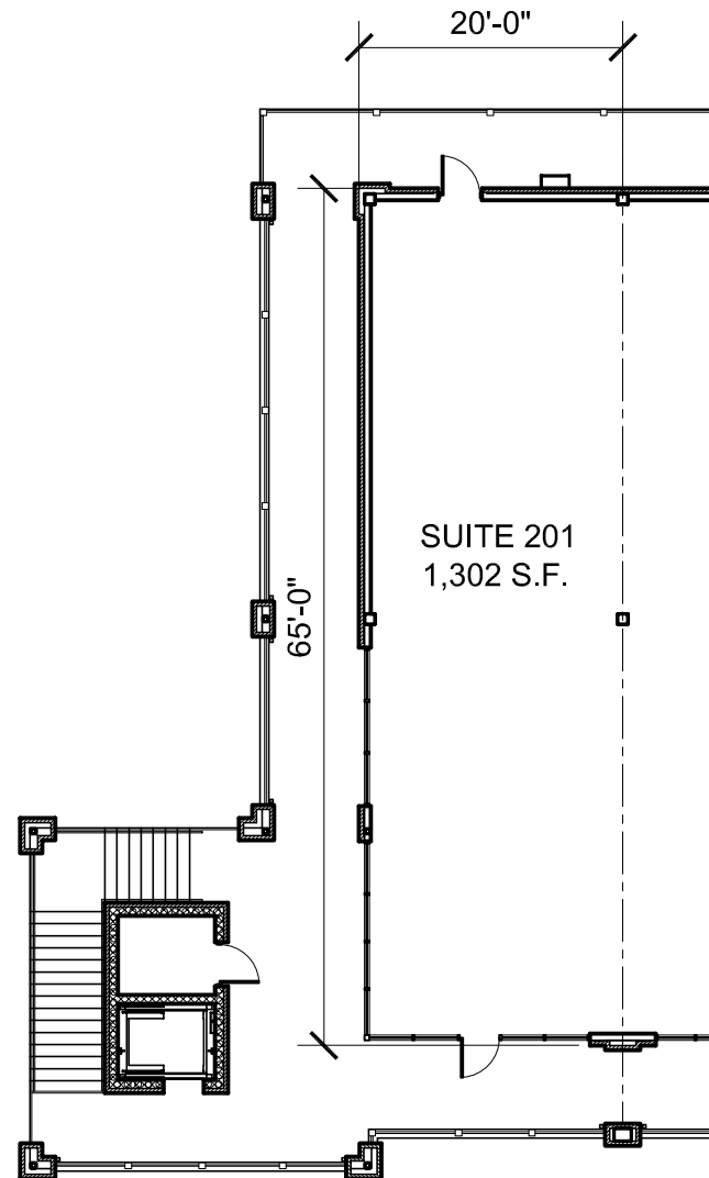
LEASING PLAN - SUITE 201
