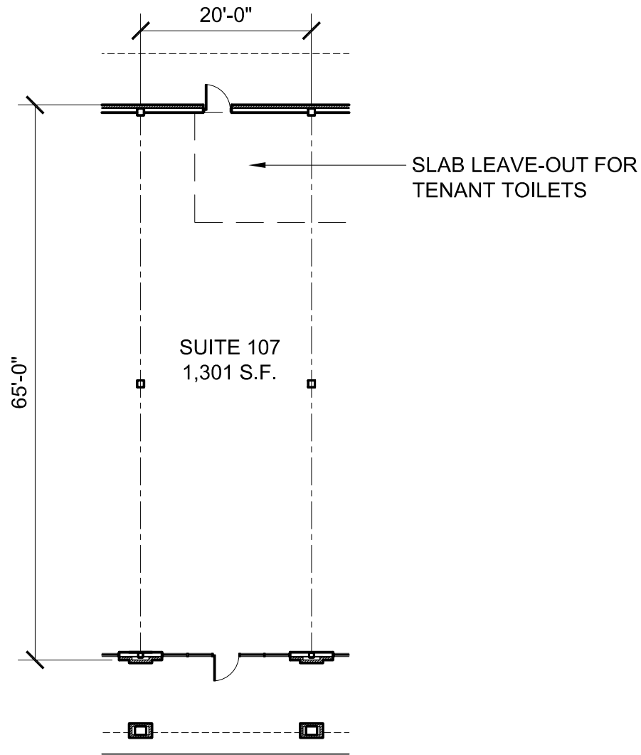
LEASING PLAN - SUITE 107
