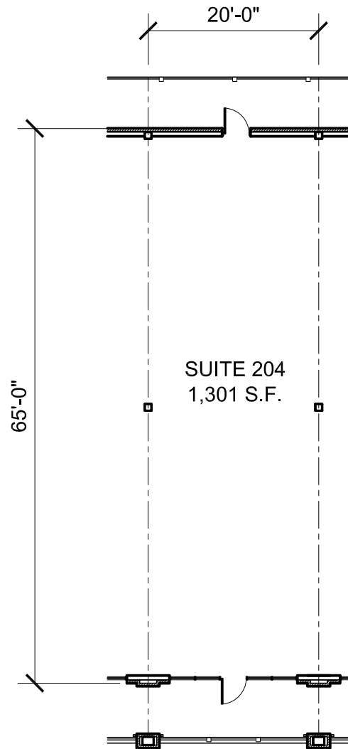
LEASING PLAN - SUITE 204
