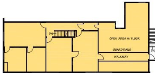
OFFICE 2ND FLOOR PLAN SCALE: 1"=20'-0"
