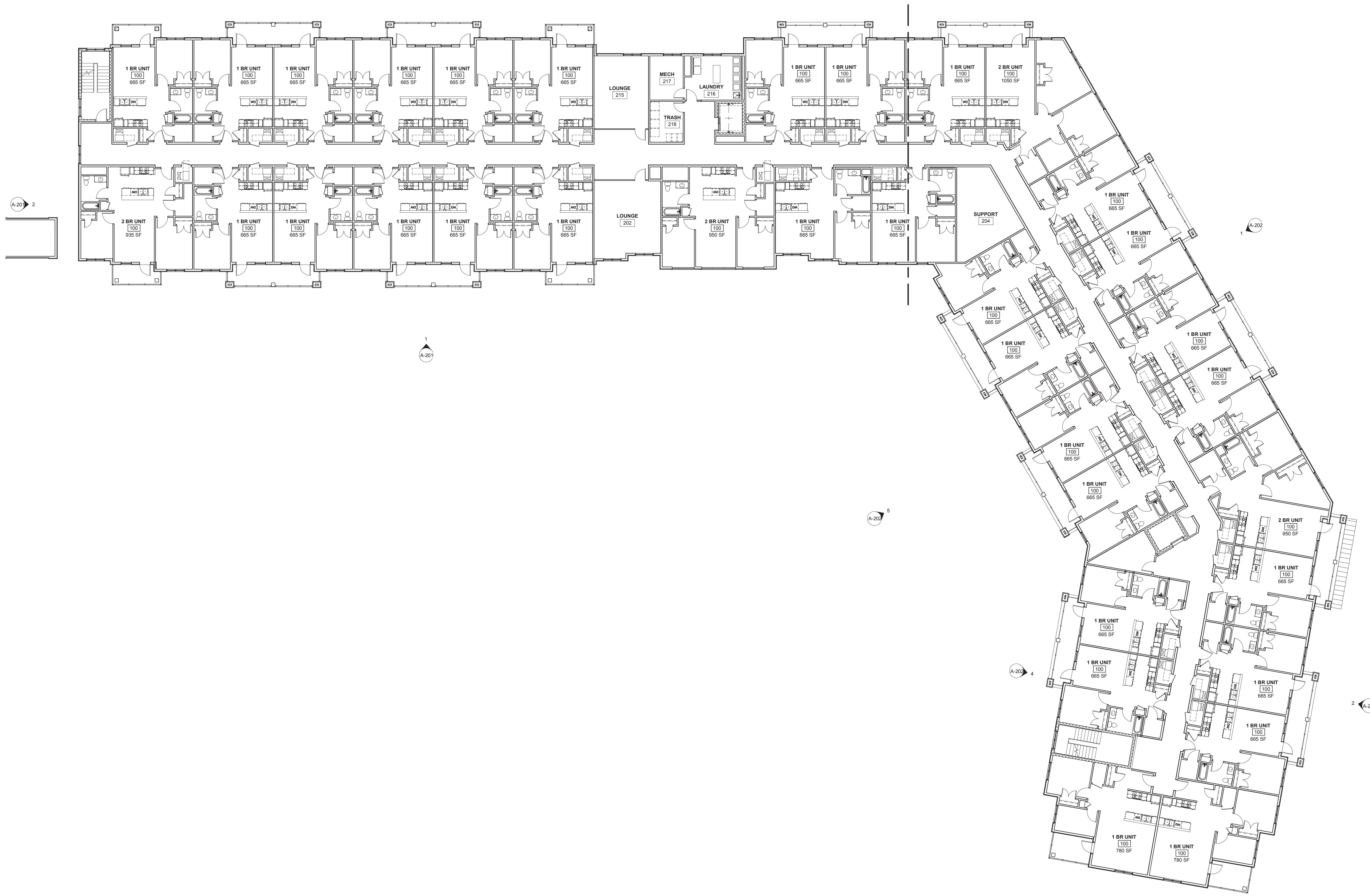
1 Third Floor Plan - Overall 3/32" = 1'-0"
