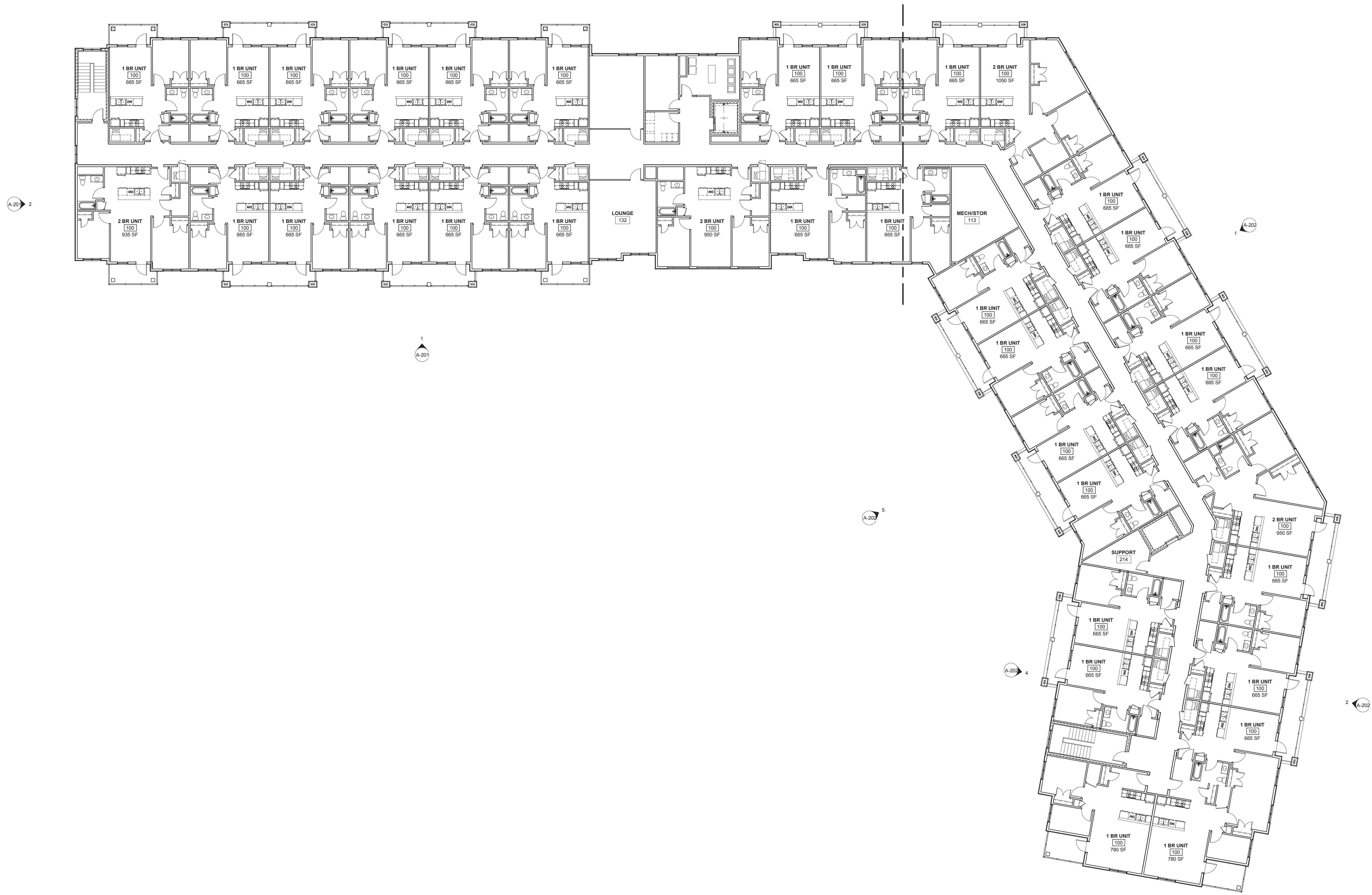
1 04th Floor Plan - Overall 3/32" = 1'-0"
