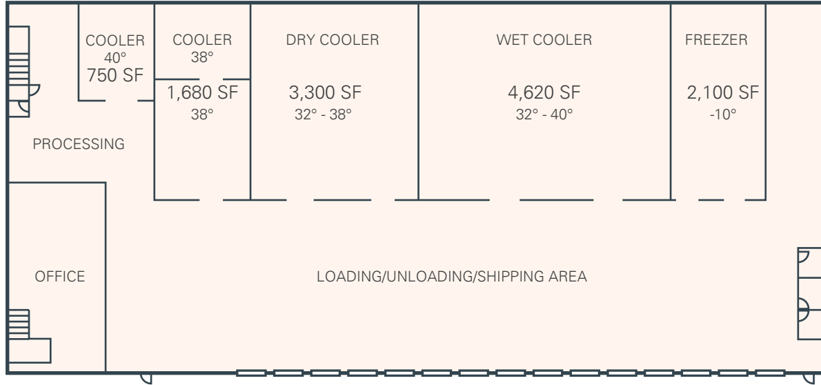
FLOOR PLAN
