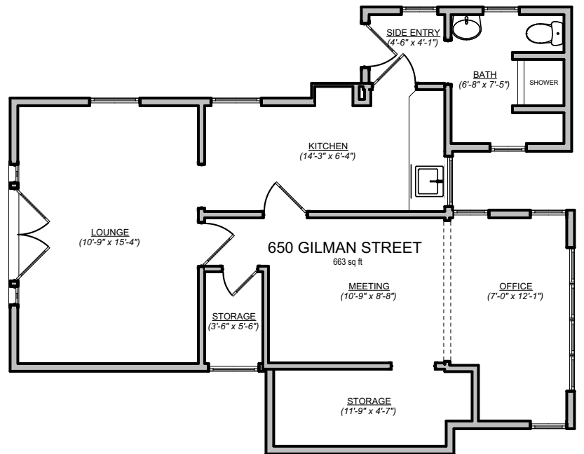
STUDIO PLAN 1/8" = 1'-0"
