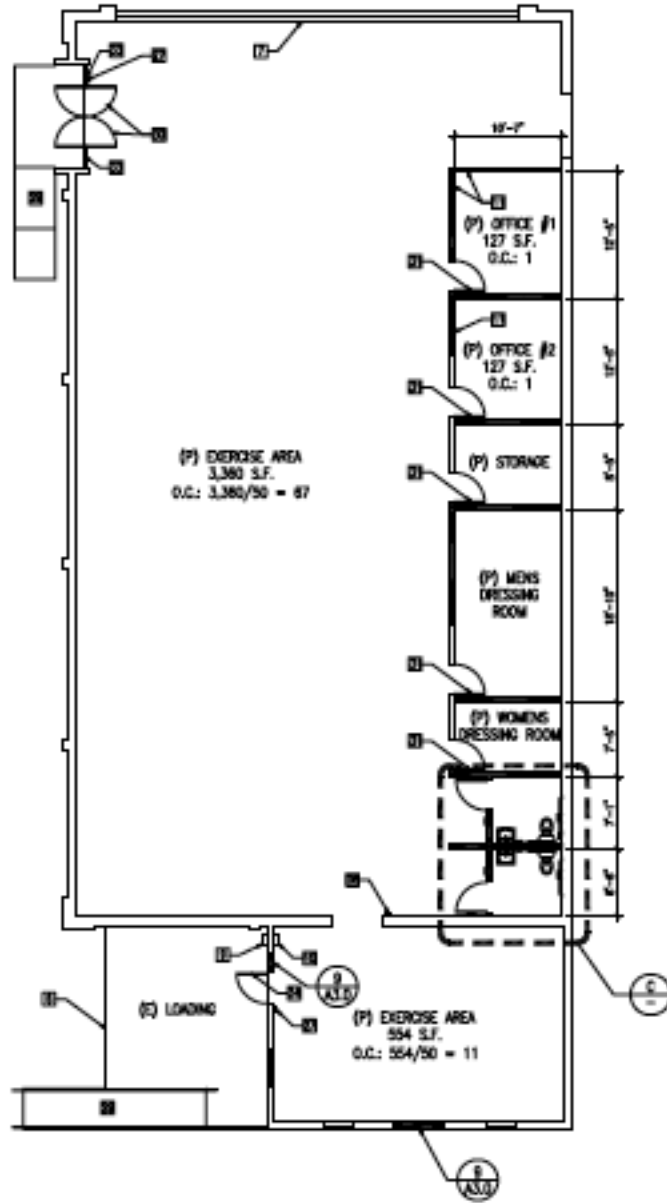
PROPOSED FLOOR PLAN SCALE 1/8" = 1'-0"
