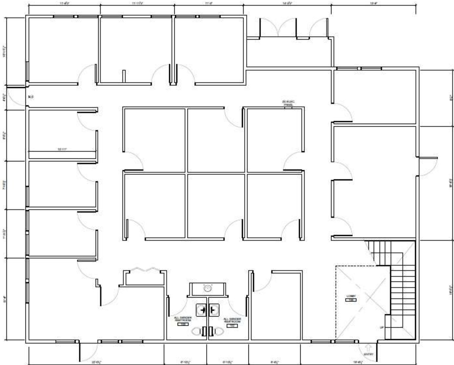
1 EXISTING 1ST FLOOR PLAN 1/8" = 1'-0"
