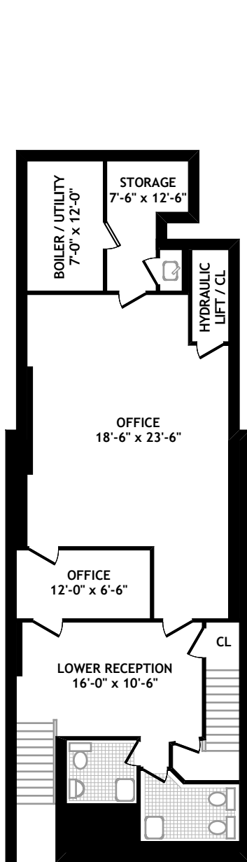
LOWER LEVEL
