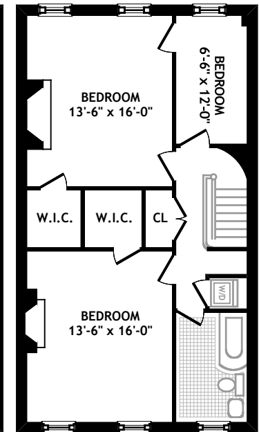
FOURTH FLOOR
