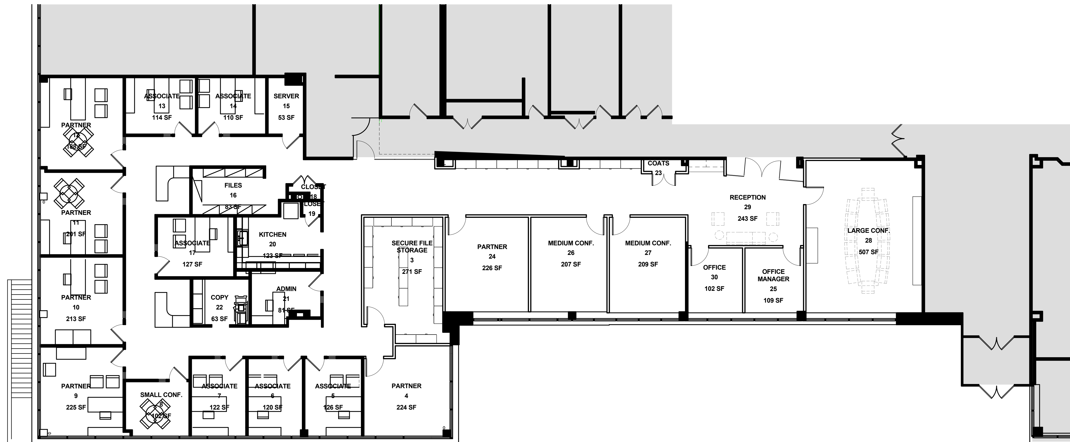
1 FIRST FLOOR SPACE PLAN OPT 2 1/8" = 1'-0"
