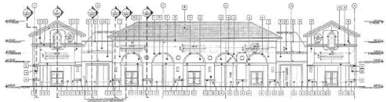
05 NORTH ELEVATION SCALE: 1/8"=1'-0"
