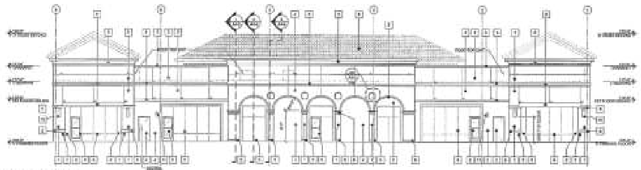
07 SOUTH ELEVATION SCALE: 1/8"=1'-0"
