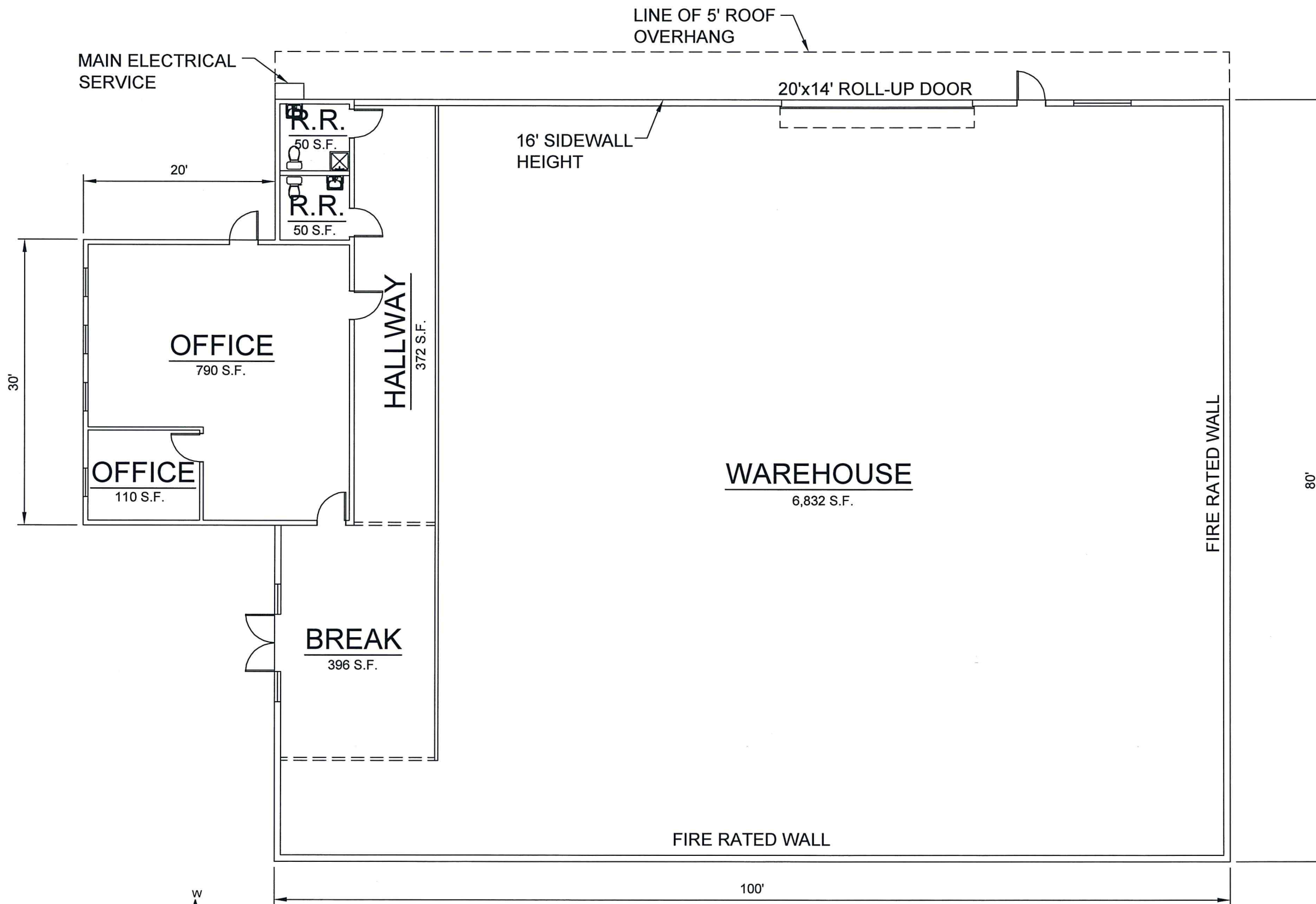
FLOOR PLAN 8,600 S.F. 2801 LASITER LANE, TURLOCK
